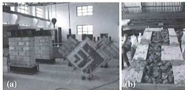
Fig. 1 a Three-leaf stone masonry wallettes, simulating the masonry of the Katholikon of Dafni Monastery and b the infill material
