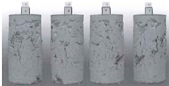
Fig. 5 Typical failure mode of injected cylinders
