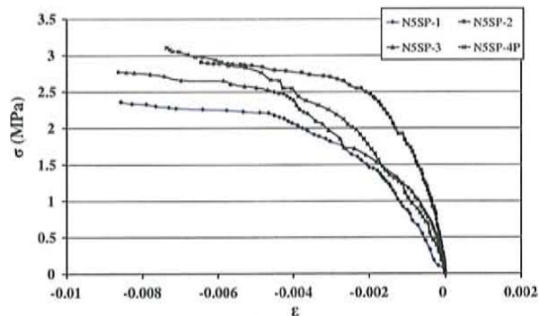
Fig. 4 Typical stress-strain curves (cylinders injected with grout G2)
